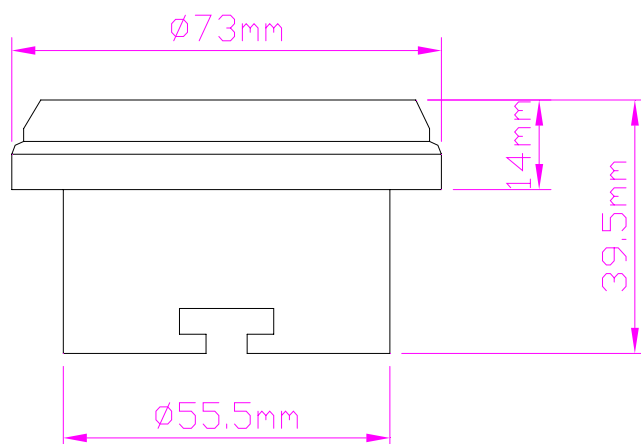
Figure 0 Product Dimensions
