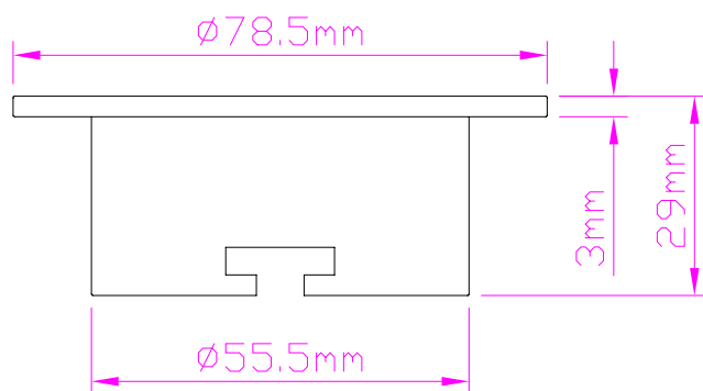
Figure 0 Product Dimensions
